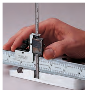
Measuring depth
