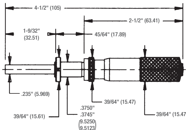
263L-38TN, 0-1" dimensions
