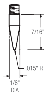
PT25161 Cone Contact Point
