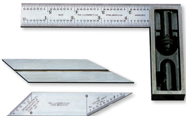
13F Double Square complete with graduated blade, beveled blade, and drill grinding blade.
