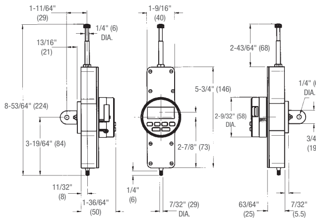
2"/50 mm Models
