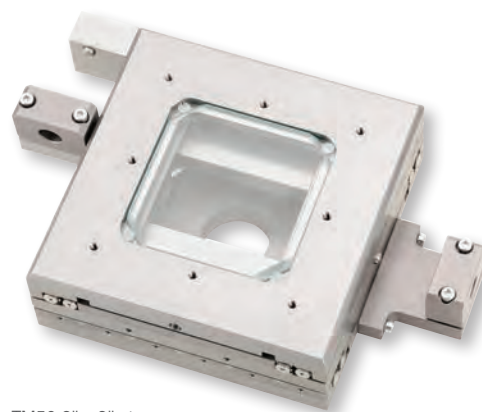
TM50 2" x 2" stage
