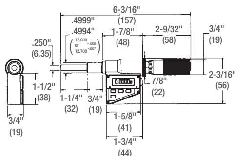
0-1" (0-25mm) dimensions
