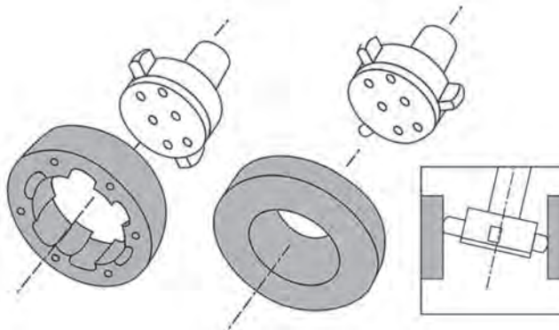
2-point and 3-point spherical radius heads are available
