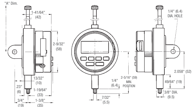
1"/25mm Models
