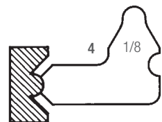
Fig 4. Checking convex (external) radius with arc of 90° or greater, or radii with sides as shown which would interfere with gage used as in Fig. 3.
